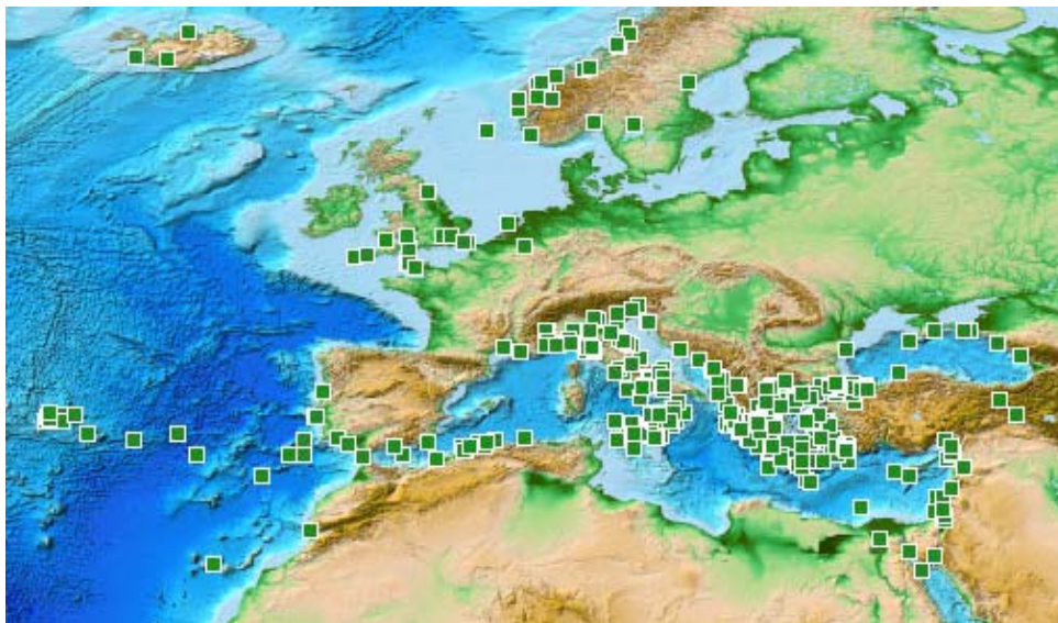
Fig. 1.1. Locations of all recorded tsunami events in the NEAMTWS region.
